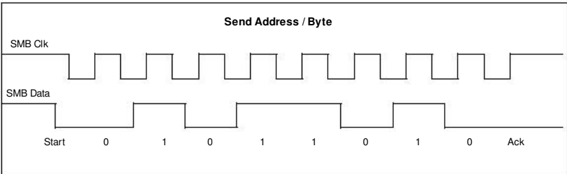
FIGURE 6 - SAMPLE SMBUS SINGLE BYTE TRANSACTION
