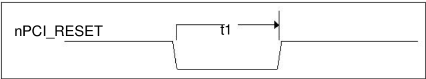
FIGURE 8C - RESET TIMING
