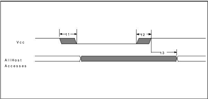
FIGURE 7 - POWER-UP TIMING
