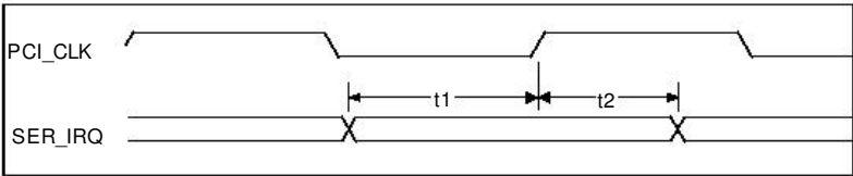
FIGURE 29 – SETUP AND HOLD TIME
