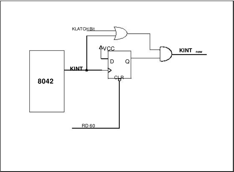
FIGURE 3 - KEYBOARD LATCH
