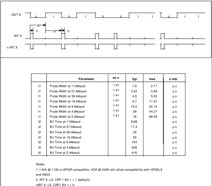
FIGURE 25 - IrDA TRANSMIT TIMING
