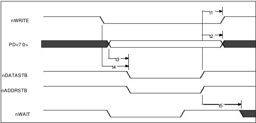
FIGURE 19 – EPP 1.7 DATA OR ADDRESS WRITE CYCLE
