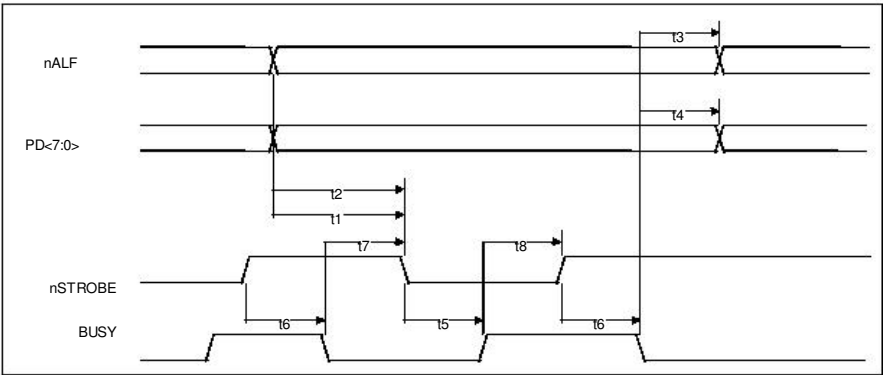
FIGURE 22 - ECP PARALLEL PORT FORWARD TIMING
