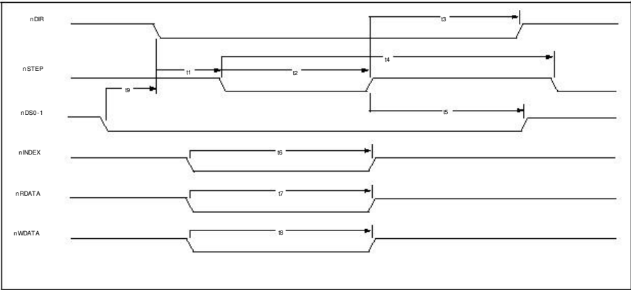
FIGURE 16 – FLOPPY DISK DRIVE TIMING (AT MODE ONLY)
