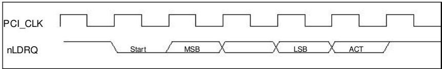
FIGURE 13 – DMA REQUEST ASSERTION THROUGH nLDRQ
