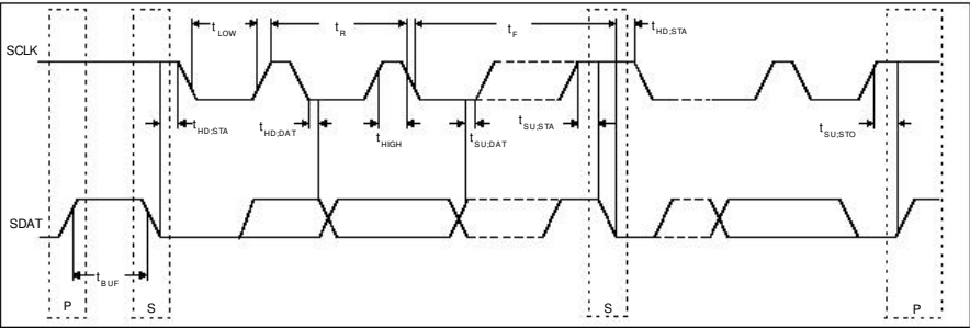
FIGURE 28 - SMBUS TIMING
