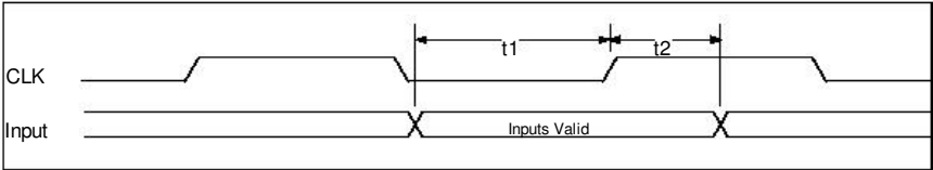
FIGURE 10 – INPUT TIMING MEASUREMENT CONDITIONS, LPC SIGNALS
