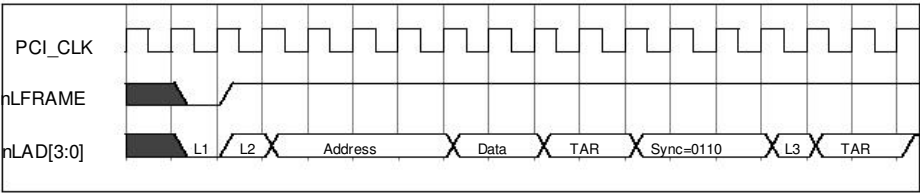
FIGURE 11 – I/O WRITE Note: L1=Start; L2=CYCTYP+DIR; L3=Sync of 0000
