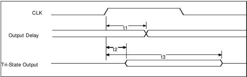
FIGURE 9 – OUTPUT TIMING MEASUREMENT CONDITIONS, LPC SIGNALS
