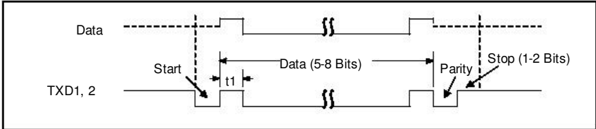
FIGURE 30 – SERIAL PORT DATA
