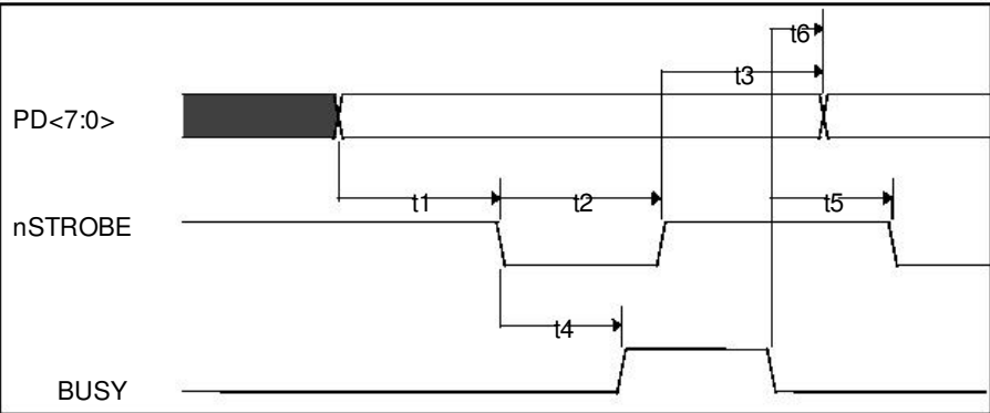
FIGURE 21 - PARALLEL PORT FIFO TIMING
