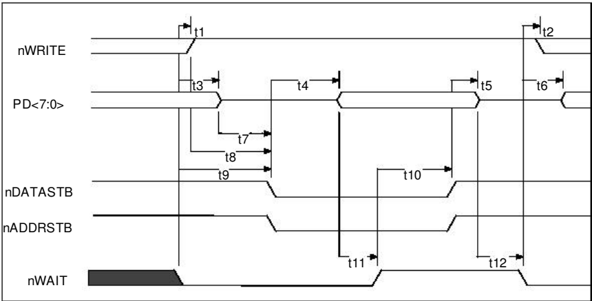
FIGURE 18 – EPP 1.9 DATA OR ADDRESS READ CYCLE
