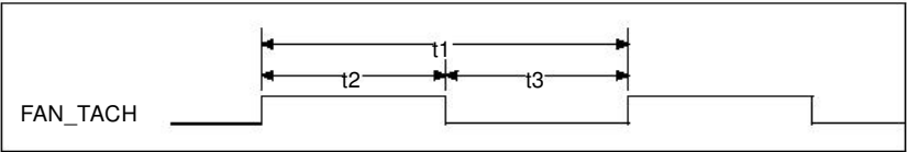
FIGURE 33 – FAN TACHOMETER INPUT TIMING
