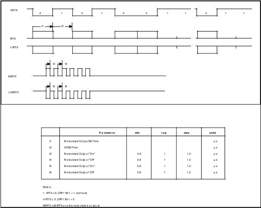
FIGURE 27 - AMPLITUDE SHIFT KEYED IR TRANSMIT TIMING
