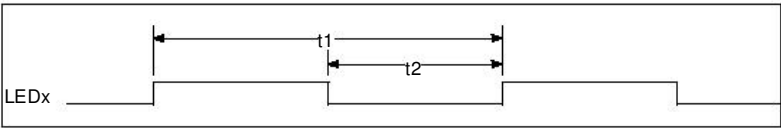
FIGURE 34 – LED OUTPUT TIMING
