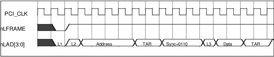
FIGURE 12 – I/O READ Note: L1=Start; L2=CYCTYP+DIR; L3=Sync of 0000
