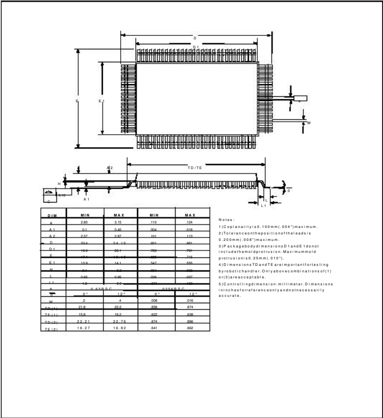
FIGURE 35 - 100 PIN QFP PACKAGE OUTLINE
