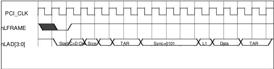
FIGURE 14 – DMA WRITE (FIRST BYTE)
