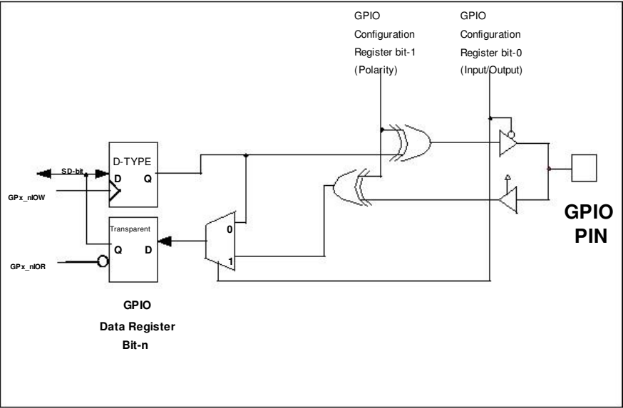
FIGURE 5 - GPIO FUNCTION ILLUSTRATION
