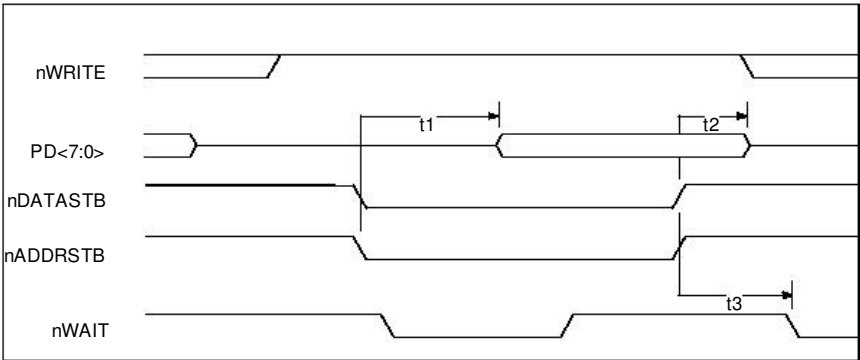
FIGURE 20 – EPP 1.7 DATA OR ADDRESS READ CYCLE
