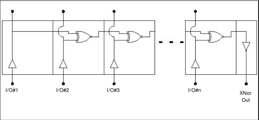
FIGURE 36 – XNOR-CHAIN TEST STRUCTURE
