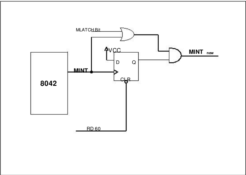
FIGURE 4 – MOUSE LATCH
