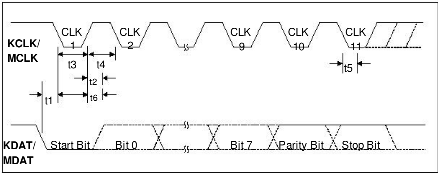
FIGURE 31 – KEYBOARD/MOUSE RECEIVE/SEND DATA TIMING
