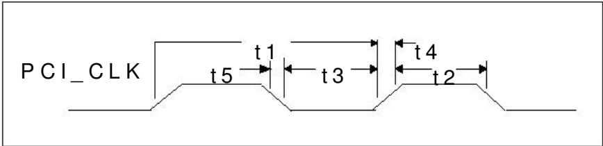
FIGURE 8B – PCI CLOCK TIMING
