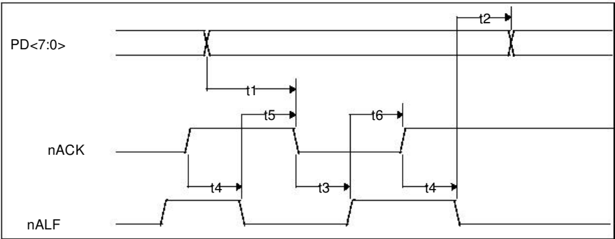
FIGURE 23 - ECP PARALLEL PORT REVERSE TIMING
