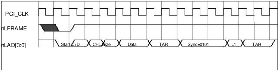
FIGURE 15 – DMA READ (FIRST BYTE)
