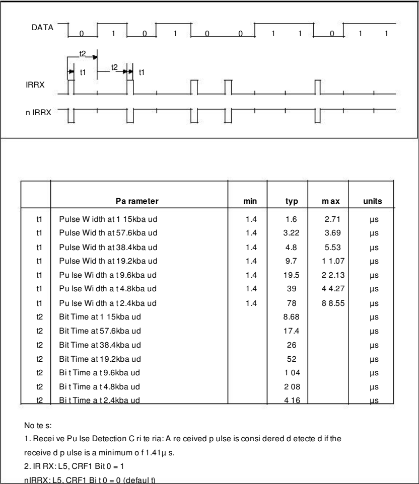
FIGURE 24 - IrDA RECEIVE TIMING
