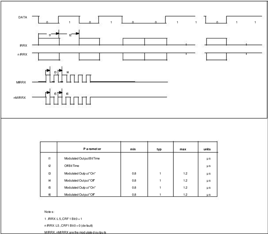
FIGURE 26 - AMPLITUDE SHIFT KEYED IR RECEIVE TIMING
