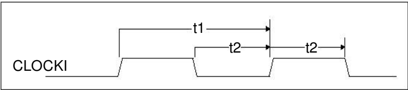
FIGURE 8A - INPUT CLOCK TIMING
