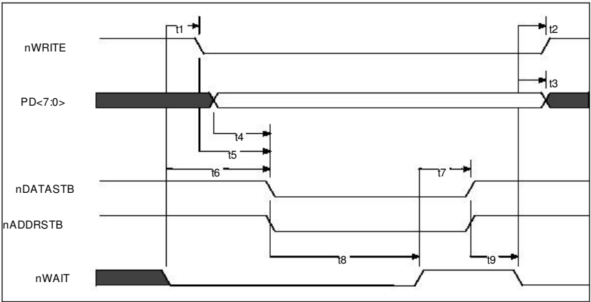
FIGURE 17 – EPP 1.9 DATA OR ADDRESS WRITE CYCLE
