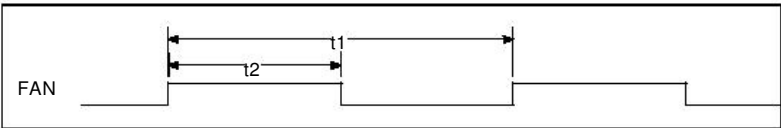
FIGURE 32 – FAN OUTPUT TIMING
